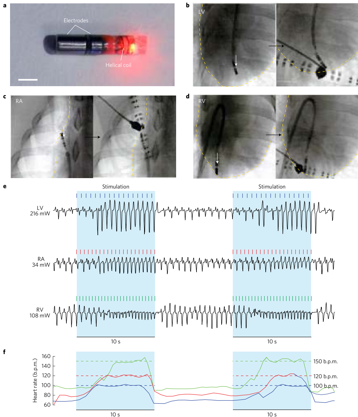
Figure 5 | In vivo wireless cardiac pacing in fig. a , Microdevice configured as a cardiac stimulator. Scale bar, 2 mm. b-d , Projection X-ray images of the stimulator (white arrow) inserted by catheter in the left ventricle (LV, b ), right atrium (RA, c ) and right ventricle (RV, d ) of the heart. For each pair, the image on the right shows the phased surface placed on the chest. Dashed yellow lines show the contours of the heart. e , Electrocardiogram recording during 10 s stimulation and rest cycles. Stimulation pulse width, 10 ms; period, 600 ms (LV), 500 ms (RA) and 400 ms (RV); average power, 216 mW (LV), 34 mW (RA) and 108 mW (RV). f , Heart rate during stimulation and rest cycles. Dotted lines show the target heart rate.
